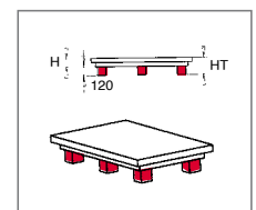
Lower frame with fork pockets
